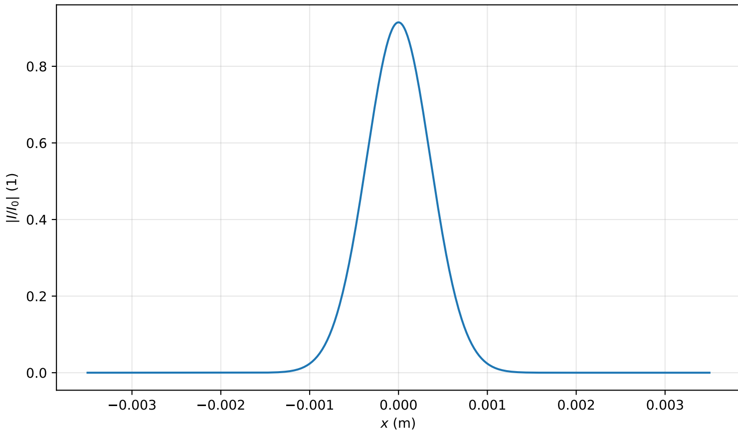
Intensity profile I(x, y = 0, z = 0.716m)/I_0 , P_{in}=0.1P_{cr} , artificial time
